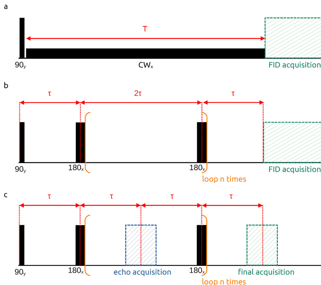
Fig. 1. (a) SLIC: Spin-locking is applied for the total time T , followed by FID acquisition. (b) Synchronized echo (SyncE) with a single acquisition: For a series of \tau values, a train of refocusing pulses is played out followed by an FID acquisition. Delay \tau and number of loops n are chosen so that the total time for the echo train, T = 2\tau(n + 1) , is always the same. (c) Multi-acquisition synchronized echo: Measurements of echo intensity are acquired within the pulse train, followed by an optional acquisition of the final echo and/or FID.
