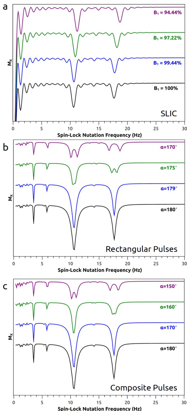
Fig. 6. Simulated effects of B_1 imperfections on the J-coupling spectrum of hydrated ethanol. (a) SLIC with B_1 errors between 0 and 5.56%. (b) Multi-acquisition synchronized echo using rectangular refocusing pulses with pulse angle errors between 0 and 10, corresponding to B_1 offsets between 0 and 5.56%. (c) Multi-acquisition synchronized echo using 90_y-180_x-90_y composite refocusing pulses with pulse angle errors between 0 and 30, corresponding to B_1 offsets between 0 and 16.68%.
