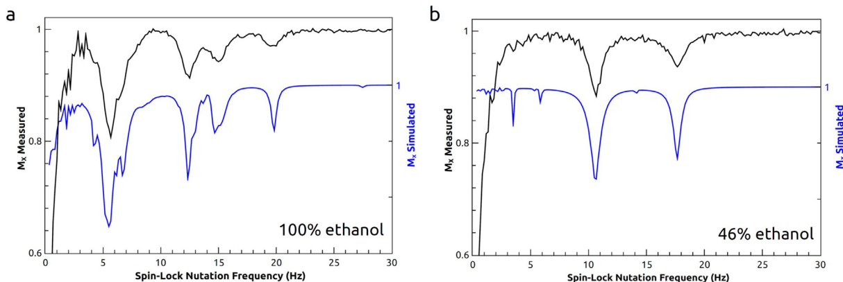
Fig. 4. Measured (black) and simulated (blue) J-coupling spectra of (a) neat anhydrous ethanol and (b) a mixture of 46% ethanol and 54% deionized water (%w/w). Spectra were acquired with the multi-acquisition SyncE scheme and all echoes were averaged to create the 1D projection. All data were acquired at 276 kHz (6.5 mT).
