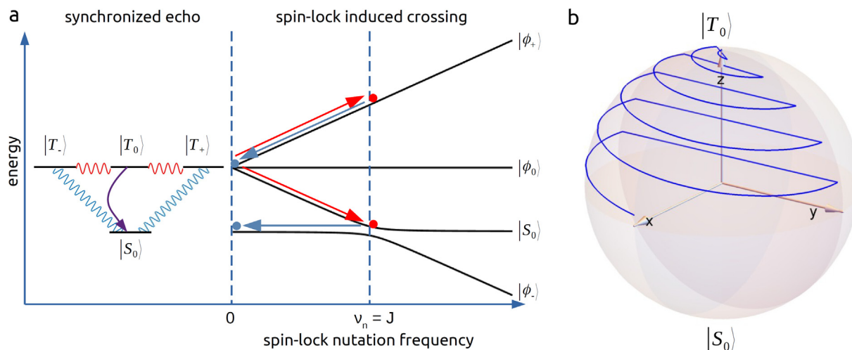
Fig. 2. (a) The synchronized echo (SyncE) sequence converts M_x , a coherence among triplet states (red), into a singlet-triplet coherence (blue), which is NMR silent. M_x can be completely depleted as it is fully transformed to the singlet-triplet coherence. On the other hand, in SLIC M_x is represented as a population of two spin-locked triplet states (red dots). During spin-locking, the population of one of these states is converted to singlet, so at the end of the sequence 50% of M_x is depleted (blue dots). The other half of M_x can also be depleted via a second block of spin-locking with the opposite phase. (b) J-synchronized echoes convert the |T_0 \rangle component to |S_0 \rangle in a series of stages around the Bloch sphere.
