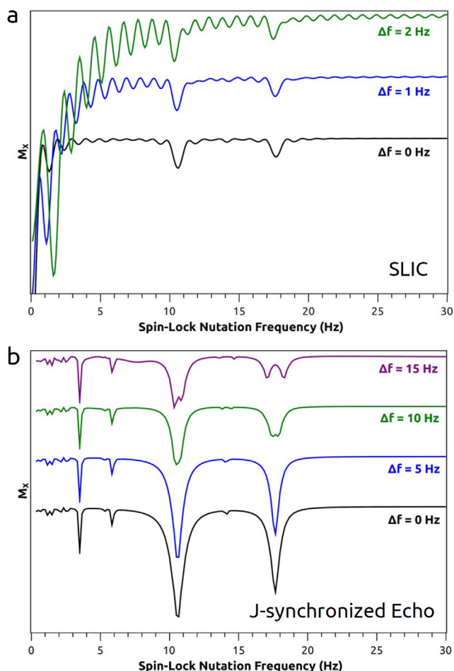
Fig. 5. Simulated effects of B_0 imperfections on the J-coupling spectrum of hydrated ethanol. (a) SLIC with B_0 offsets between 0 and 2 Hz, using a T = 1 s evolution time. (b) Multi-acquisition synchronized echo with B_0 offsets between 0 and 15 Hz, using 2 ms refocusing pulses and a T = 3 s evolution time.
