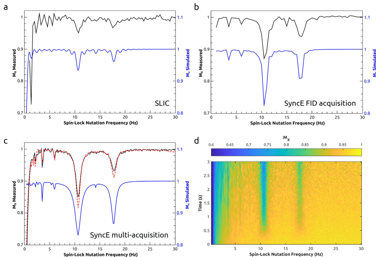
Fig. 3. Measured (black) and simulated (blue) J-coupling spectra of neat ethyl acetate acquired with (a) SLIC, (b) synchronized echo (SyncE) using FID acquisitions, and (c) SyncE using the multi-acquisition scheme and averaging echoes. For the red dotted trace the hard pulses of the echo train were replaced with composite pulses. (d) 2D spectrum of ethyl acetate acquired with the multi-acquisition SyncE scheme. All data were acquired at 276 kHz (6.5 mT).
